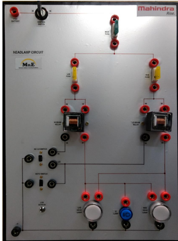
FRONT VIEW
