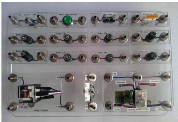
Test Fixture-A
